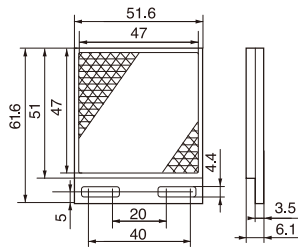
P250F (Standard, ZR-QX200)
