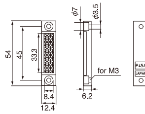
Tiny reflector P45A (Optional, LED type)
